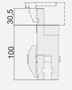
American Type Mechanical Punch Clamping
