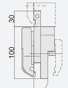
Euro Type Pneumatic Punch Clamping
